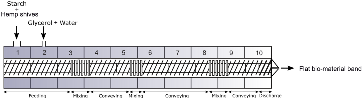
Figure 1. Schematic illustration of the extruder barrel, with its 10 zones of temperature control, and screw profile.
