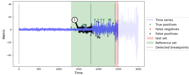
Figure 28: Examples of failure of anomaly detection on time series with change in the variance.
