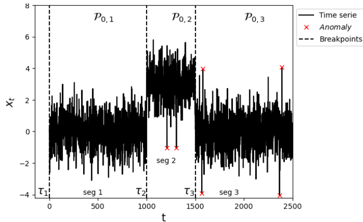
Figure 2: Illustration of piecewise stationary time series.
