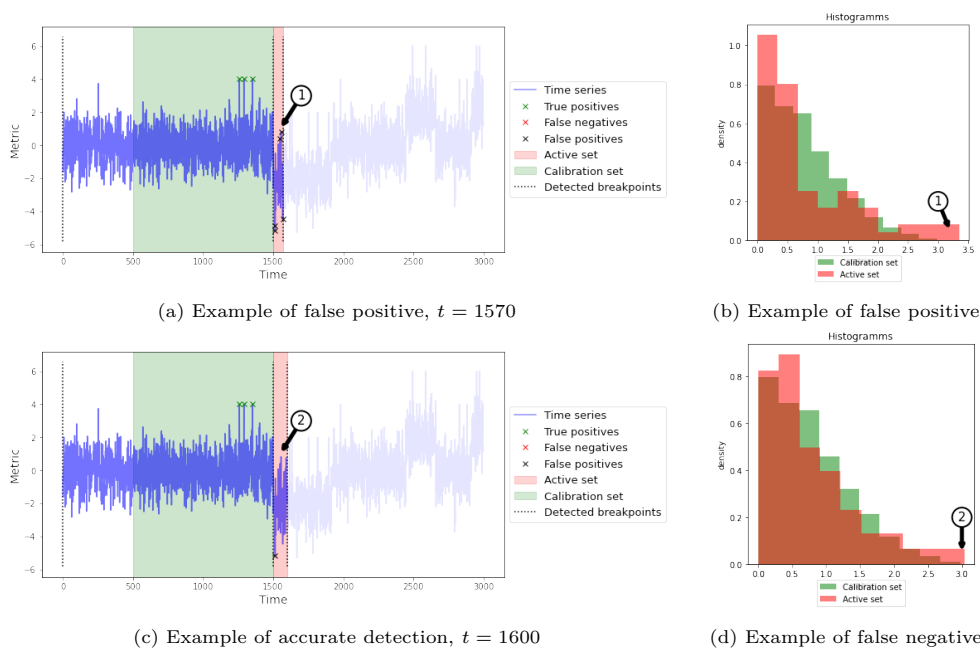
Figure 31: Abnormality status update after new data points acquisition in the current segment.
