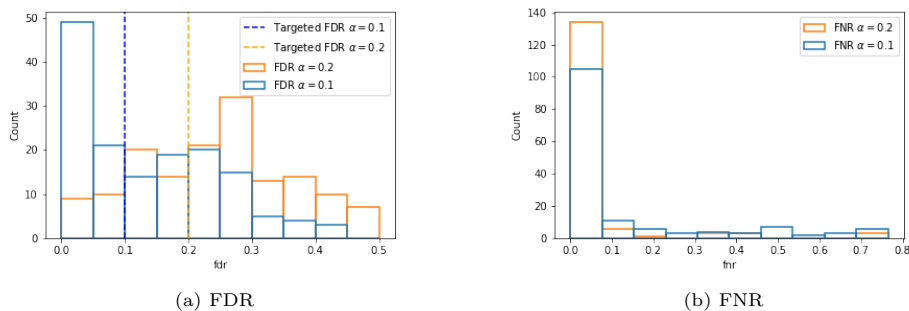
Figure 18: Histograms of the FDR and FNR for different targeted FDR \alpha levels.
