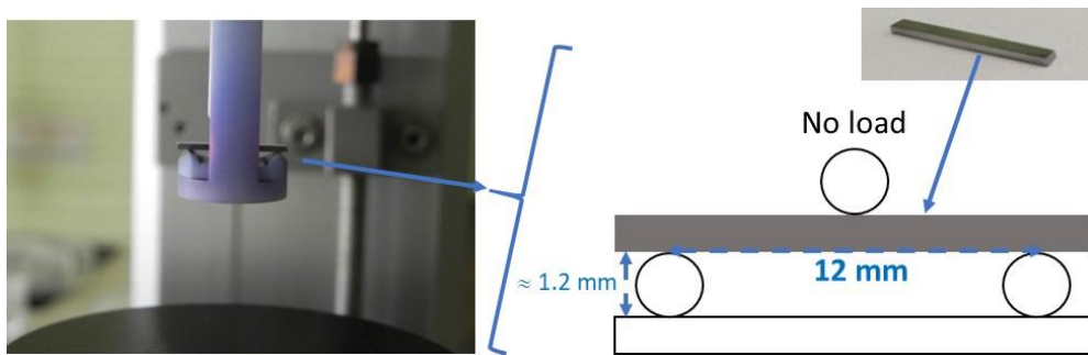
Fig. 1. Photograph of the sample positioned in the alumina device taken prior to chamber closing (left) and principle of the three points flexural test before applying the load (right).
