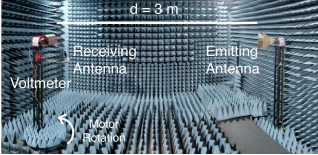
Fig. 13. Measurement setup in the anechoic chamber.
