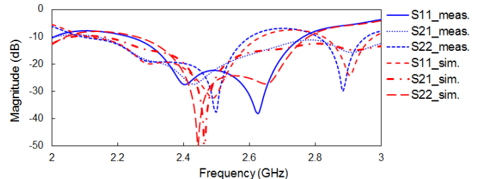
Fig. 7. Simulated and measured reflection and isolation coefficients (dB) of ports 1 and 2 of the Butler matrix.
