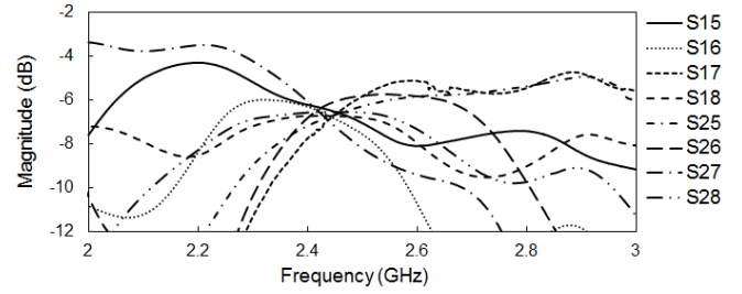
Fig. 5. Simulated amplitudes (dB) in transmission from ports 5,6,7 and 8 to ports 1 and 2 of the Butler matrix. Transmissions to ports 3 and 4 are similar to those to ports 1 and 2 due to the symmetry of the matrix.
