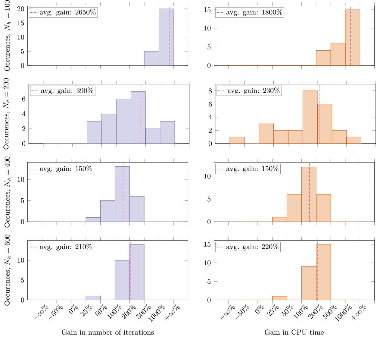
Figure 6: Statistics of the gains G_{\text{iter}} in number of iterations (left panels) and G_{\text{CPU}} in CPU time (right panels) for the 1D problem (1.2) with \alpha_0 = 5 . From top to bottom, we display the results for meshes with 100, 200, 400 and 600 points. The gains are grouped in bins of varying sizes, and the number of occurrences in each bin is displayed as a histogram.
