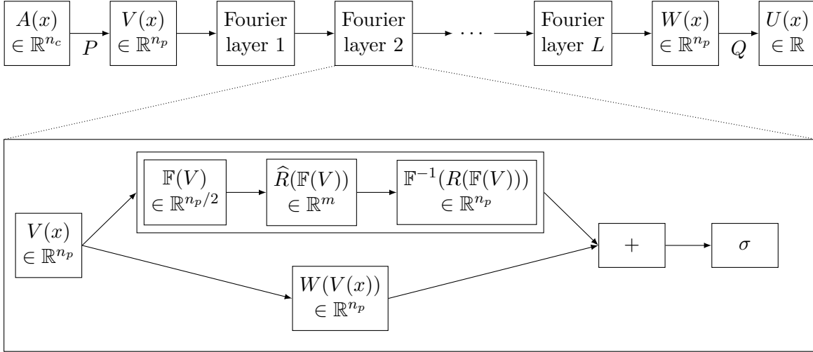
Figure 1: Sketch of an FNO, adapted from [34]. The network has n_c input channels ( n_c = 2 in 1D and n_c = 5 in 2D), which are then extrapolated to n_p dimensions by the extrapolation layer P ; L Fourier layers follow, whose result is projected back to \mathbb{R} to give an approximation of the PDE solution. In the Fourier layers, \mathbb{F} denotes the fast Fourier transform FFT.
