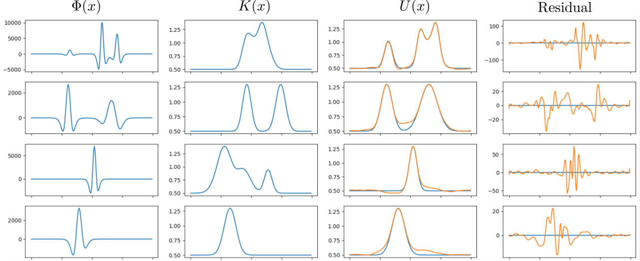
Figure 4: Examples obtained after training the FNO with the loss function \mathcal{L}_{\text{data}}^{L^2} from (2.4) and the discretization-informed loss function \mathcal{L}_{\text{dis}} from (2.6). From top to bottom, the four graphs correspond to a different example. In the first three columns, from left to right, we display \Phi(x) , K(x) , the solution U(x) (blue line) and its prediction (orange line). The rightmost column compares the residuals of the discretized PDE computed with the exact solution (blue line) and the predicted solution (orange line).
