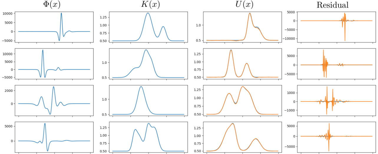
Figure 3: Examples obtained after training the FNO with the loss function \mathcal{L}_{\text{data}}^{L^2} from (2.4) only. From top to bottom, each series of graphs corresponds to a different example. In the first three columns, from left to right, we display \Phi(x) , K(x) , the solution U(x) (blue line) and its prediction (orange line). The rightmost column compares the residuals of the discretized PDE computed with the exact solution (blue line) and the predicted solution (orange line).
