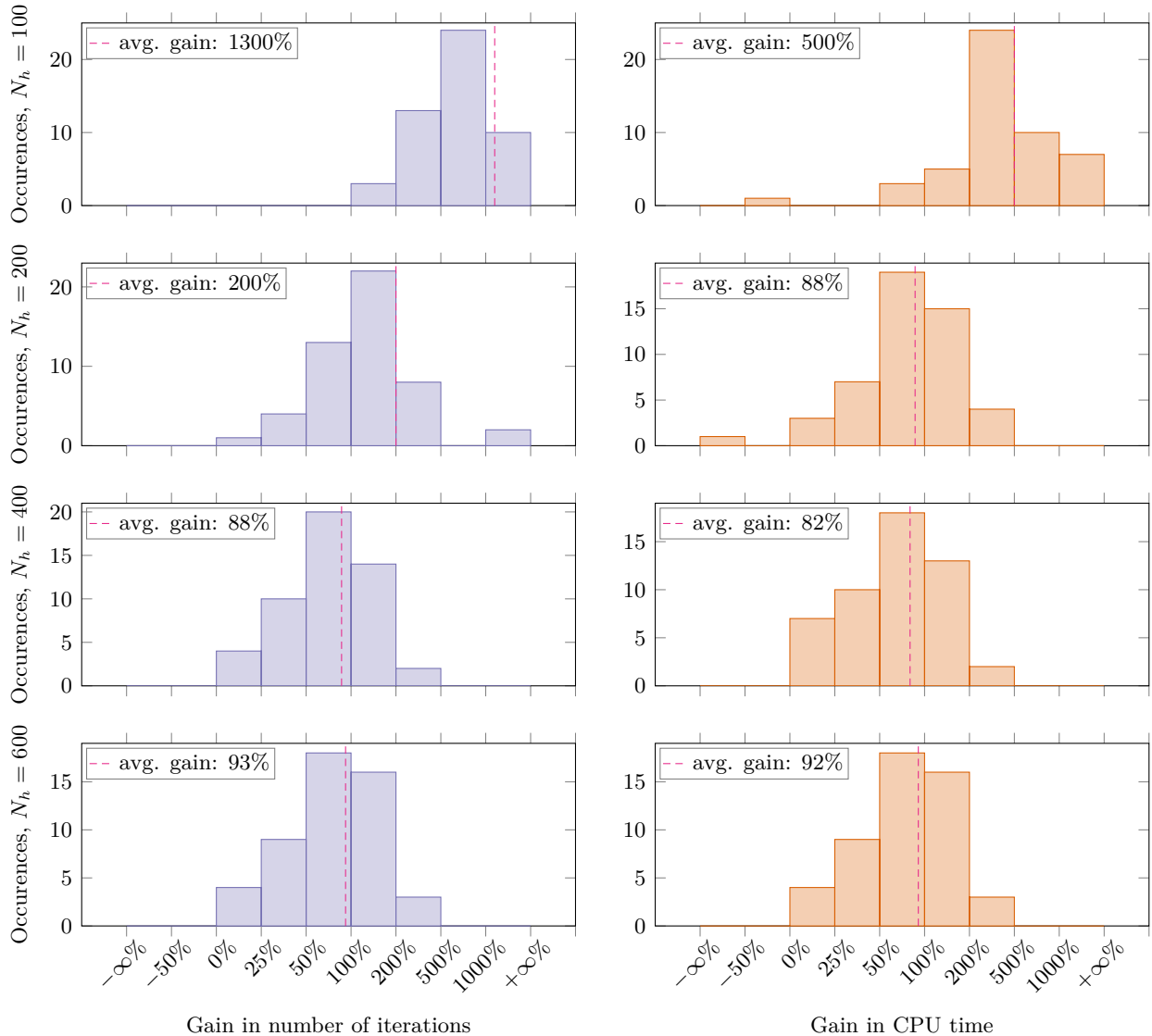
Figure 5: Statistics of the gains G_{iter} in number of iterations (left panels) and G_{CPU} in CPU time (right panels) for the 1D problem (1.2) with \alpha_0 = 2 . From top to bottom, we display the results for meshes with 100, 200, 400 and 600 points. The gains are grouped in bins of varying sizes, and the number of occurrences in each bin is displayed as a histogram.
