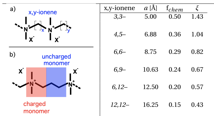
Figure 1. Left: (a) Schematic view of an x, y -ionene chain. (b) Schematic view of a 3,3-ionene ( x=3, y=3 ) chain, showing the definition of a charged and uncharged monomer. Right: Ionene structural parameters: a is the charge separation on the chain, f_{chem} the fraction of charged monomers, \xi the Manning charge density parameter, defined as \xi = L_B/a , where L_B is the Bjerrum length (7.14 Å in water at room temperature). While 4,5- ionenes are at the \xi = 1 limit (onset of Manning-type condensation), only 3,3- ionenes have sufficient charge density to induce significant condensation ( \xi > 1 ) and decrease the chemical charge ( f_{chem} ) to an effective charge ( f_{eff} ).
