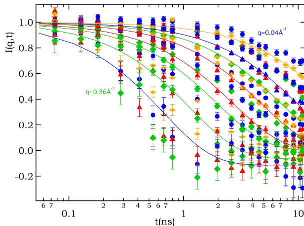
Figure 5. Intermediate scattering function, I(q, t) , measured for 6,9-Br ionene at c_p=0.4M , as measured by NSE. Each curve corresponds to a given q value in the range from 0.04 to 0.36 Å -1 . Lines are mono-exponential fits for a selection of the curves.
