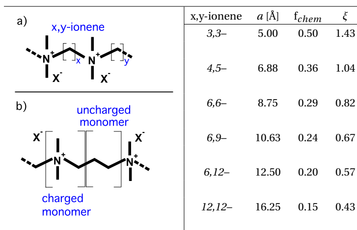
Figure 1. Left: (a) Schematic view of an x, y -ionene chain. (b) Schematic view of a 3,3-ionene ( x=3, y=3 ) chain, showing the definition of a charged and uncharged monomer. Right: Ionene structural parameters: a is the charge separation on the chain, f_{chem} the fraction of charged monomers, \xi the Manning charge density parameter, defined as \xi = L_B/a , where L_B is the Bjerrum length (7.14 Å in water at room temperature). While 4,5- ionenes are at the \xi = 1 limit (onset of Manning-type condensation), only 3,3- ionenes have sufficient charge density to induce significant condensation ( \xi > 1 ) and decrease the chemical charge ( f_{chem} ) to an effective charge ( f_{eff} ).
