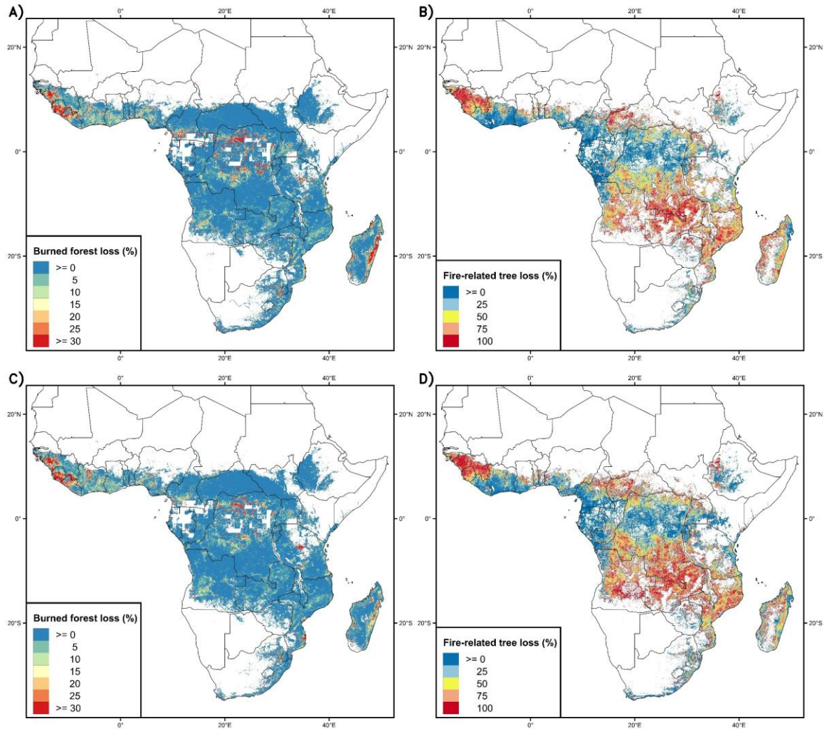
Fig. 3 | Fire impact on forest loss from FireCCISFD calculated through two parameters: the fraction of tree cover loss within burned forests in 2016 (A) and 2019 (C), and fire-related forest loss for the same years 2016 (B) and 2019 (D). The former indicates the percentage of burned area that was deforested, while the latter shows what proportion of total deforested area was fire-related.
