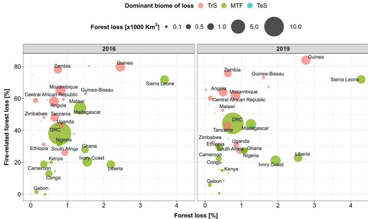
Fig. 4 | Fire-related forest loss (in proportion to total forest loss) vs total forest loss (in proportion to total forested area) across countries of SSA in 2016 and 2019. Countries with forest losses lower than 100 km 2 were not labelled. Colour of circles indicate the most affected biome by fire-related deforestation (see table A.2).
