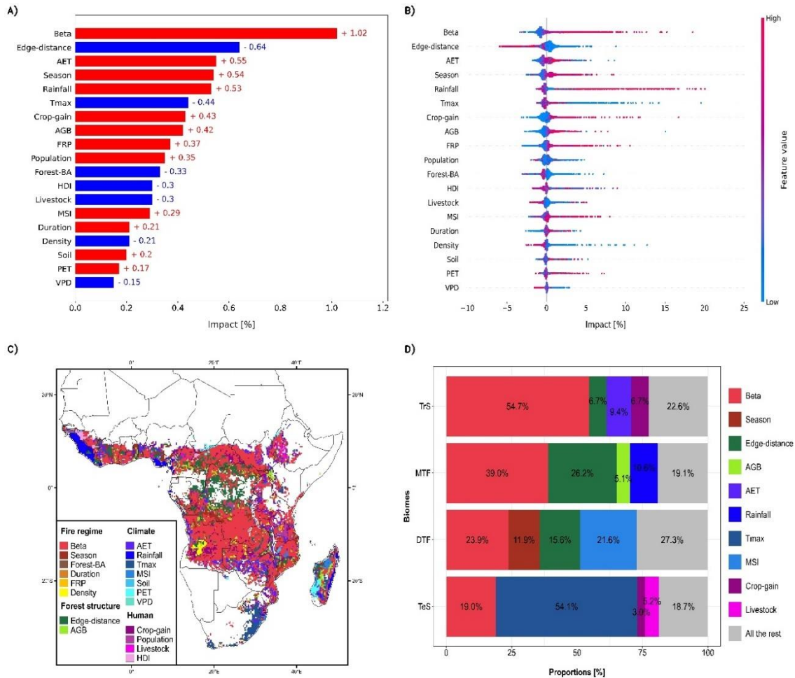
Fig. 6 | Importance of drivers of forest loss after fire in 2019. (A) The mean of absolute values of impact of each predictive variable on forest loss. The sign in association with the colour indicates the direction of impact based on the correlation with the predictions (red positive, blue negative); (B) Distribution of the predictive variable's values according to their impact on the predicted forest loss; (C) Geographical distribution of the most important predictor variables explaining forest loss per grid cell; (D) Proportions of the most important predictor variables explaining forest loss per biome. The impact values are derived from the Shapely feature importance analysis of the XGBoost model.
