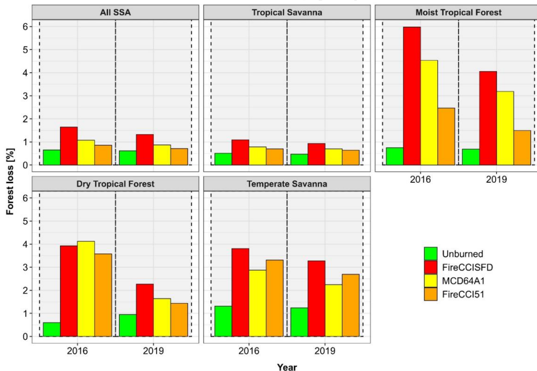
Fig. 1 | Forest loss proportions in each biome attributed to unburned and burned area (for different BA products). Unburned refers to forest areas classified as not burned in the FireCCISFD product.
