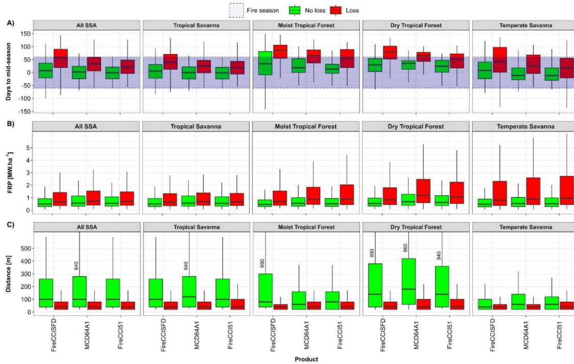
Fig. 7 | Impact of fire properties on loss or no loss of burned forests in 2019.
