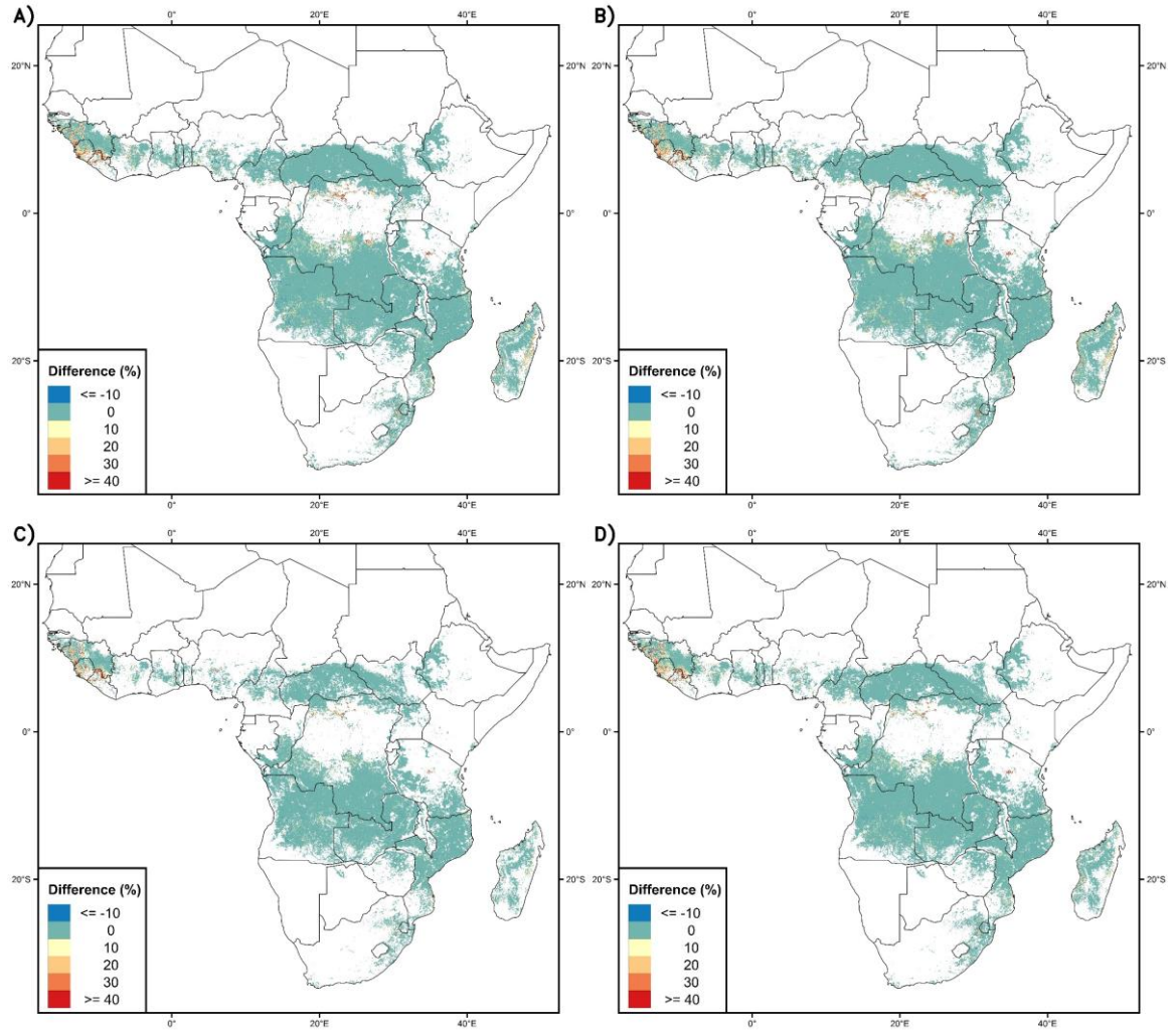
Fig. A.6 | Differences of estimations of the fraction of tree cover loss within burned forests: (A) FireCCISFD – MCD64A1 (2016); (B) FireCCISFD – FireCCI51 (2016); (C) FireCCISFD – MCD64A1 (2019); (D) FireCCISFD – FireCCI51 (2019)
