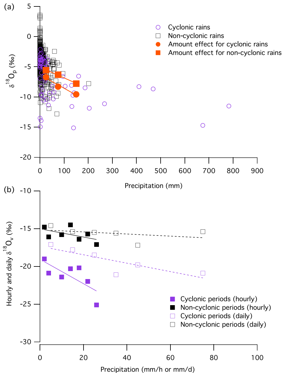
Figure 4. (a) Isotopic composition ( \delta^{18}O_p in ‰) of all rain samples as a function of precipitation amount (mm) (purple open circles are for rain occurring during cyclones and black open squares are for rain occurring outside cyclones). Orange circles (squares) are amount-weighted mean \delta^{18}O_p during (outside) cyclonic periods for three different precipitation intervals common to cyclonic and non-cyclonic periods; (b) Hourly and daily isotopic composition of water vapor ( \delta^{18}O_v in ‰) as a function of precipitation rate (mm/h and mm/d respectively) at the Piton Maïdo station for cyclonic (purple) and non-cyclonic (black) time periods. Each marker is the average of hourly or daily \delta^{18}O_v over a precipitation rate interval of 4 mm/hr and 10 mm/d respectively.
