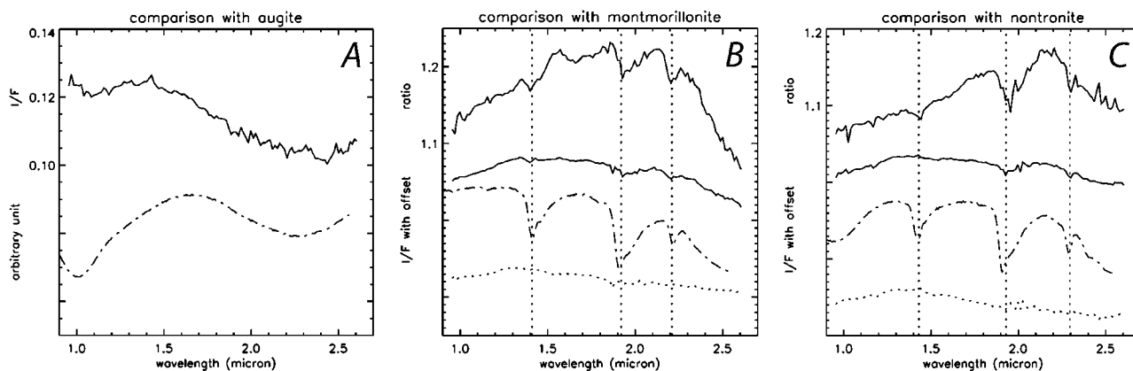
Figure 4. (a) Average of six OMEGA spectra (solid line) with pyroxene detection, compared with a laboratory spectrum of augite (clinopyroxene, dashed line, from USGS spectral library). (b and c) Smectite spectra as identified by OMEGA in the Mawrth Vallis region. (b) From bottom to top: the dotted line is the OMEGA reference spectrum; the dot-dashed line is a laboratory spectrum of montmorillonite (USGS spectral library); the bottom solid line is the average of 6 OMEGA spectra, and the top solid line is the ratio of this average over the reference spectrum. (c) The same for other pixels compared with nontronite (Fe-smectite, USGS spectral library).
