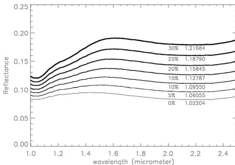
Figure 2. Synthetic spectra of intimate mixtures of high-calcium pyroxene, low-calcium pyroxene, and plagioclase mixed with varying concentrations (0%, thinnest line, to 30%, thickest line) of Mg-rich olivine of 100- \mu\text{m} grain in size. All the parameters are fixed except for the concentrations of the olivine and plagioclase (plagioclase concentration decreases when olivine concentration increases). The calculated value of the forsterite spectral parameter is indicated for each spectrum. We assume that the detection is considered positive for the OMEGA data set if the spectral parameter is larger than 1.04 (see text).
