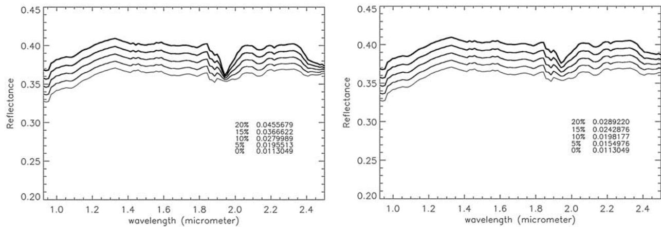
Figure 4. Synthetic spectra of intimate mixtures of gypsum and Martian-like dust for two grain sizes of gypsum: (left) 10 \mu\text{m} and (right) 5 \mu\text{m} . All the parameters are fixed except for the concentrations of the gypsum and the dust (from 0%, thinnest line, to 20%, thickest line). The dust concentration decreases when the gypsum concentration increases. The value of the 1.9- \mu\text{m} spectral parameter is indicated for each spectrum and its corresponding abundance. We assume that the detection is considered positive if the parameter is larger than 2%.
