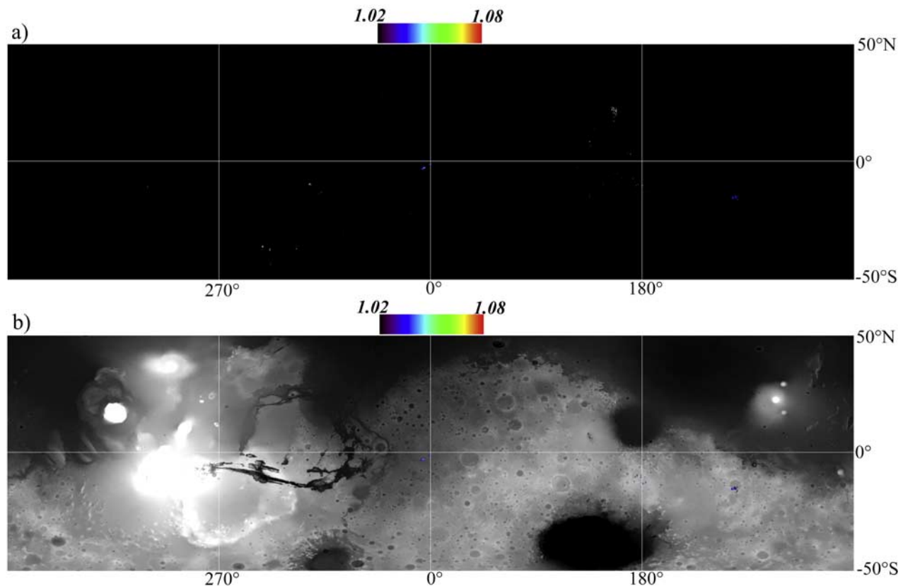
Figure 7. Same as in Figure 6 but for the fayalite parameter.
