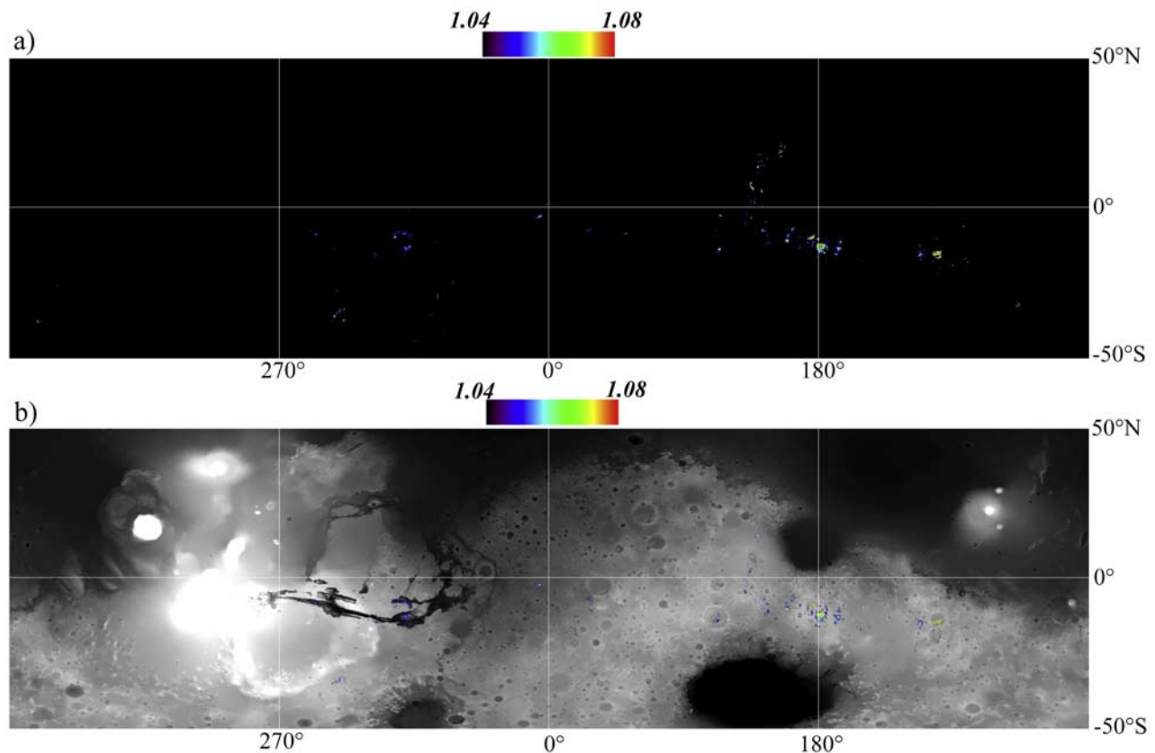
Figure 6. (a) Global distribution of forsterite parameter on a black background and (b) the MOLA altimetry. Colors that are above the scale are in white.
