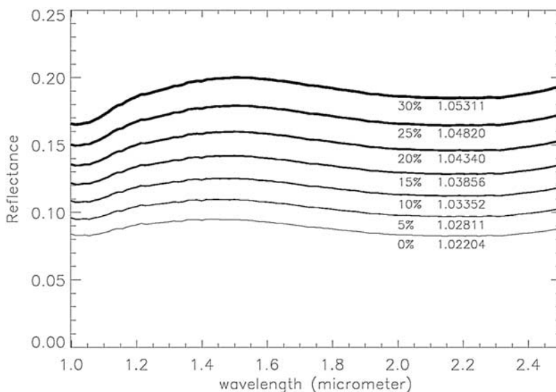
Figure 3. Same as in Figure 2 except that the grain size of the olivine component is 10 \mu\text{m} .
