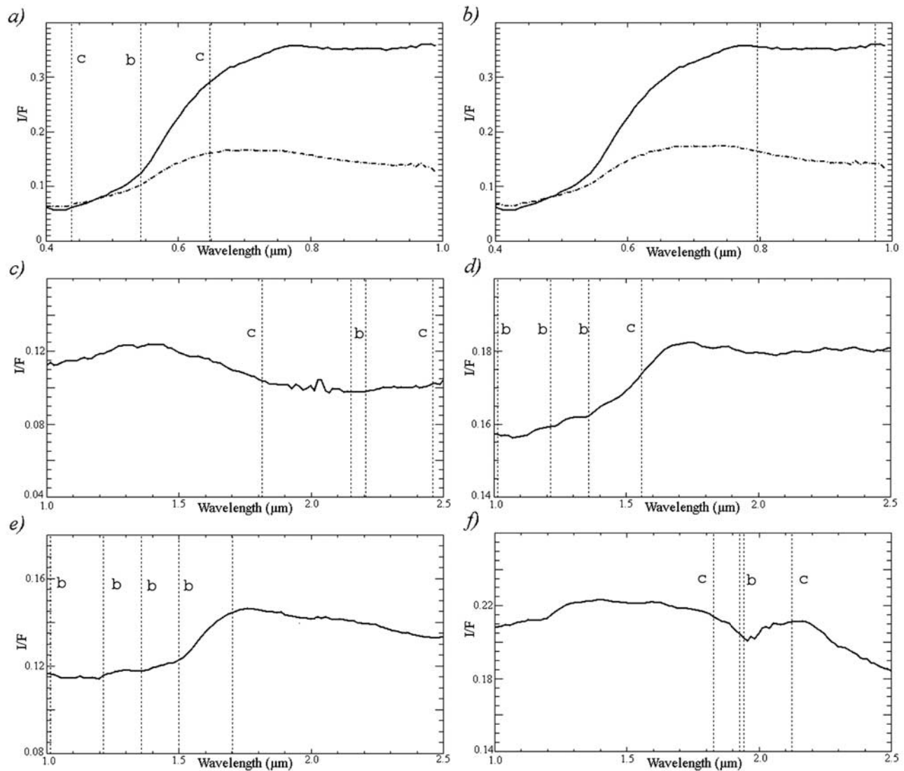
Figure 1. Band positions of spectral parameters listed in Table 1 on OMEGA spectra representative of the major spectral types discussed in the paper. (a) Fe 3+ parameter over typical spectra of dark (dashed line) and bright regions (solid line), (b) nanophase ferric oxide parameter over typical spectra of dark (dashed line) and bright regions (solid line), (c) pyroxene parameter over a typical spectrum of a pyroxene-rich terrain, (d) forsterite parameter over a spectrum of a olivine-rich (likely enriched in Mg) deposit, (e) fayalite parameter over a spectrum of a olivine-rich (likely enriched in Fe) deposit, and (f) 1.9- \mu\text{m} parameter over a spectrum of water-bearing terrains identified by the 1.9- \mu\text{m} band. The vertical dashed bars indicate the wavelengths used for the band centers (labeled by b) and the wavelengths used for the continuum (labeled by c) used in the calculation of the spectral parameters (Table 1).
