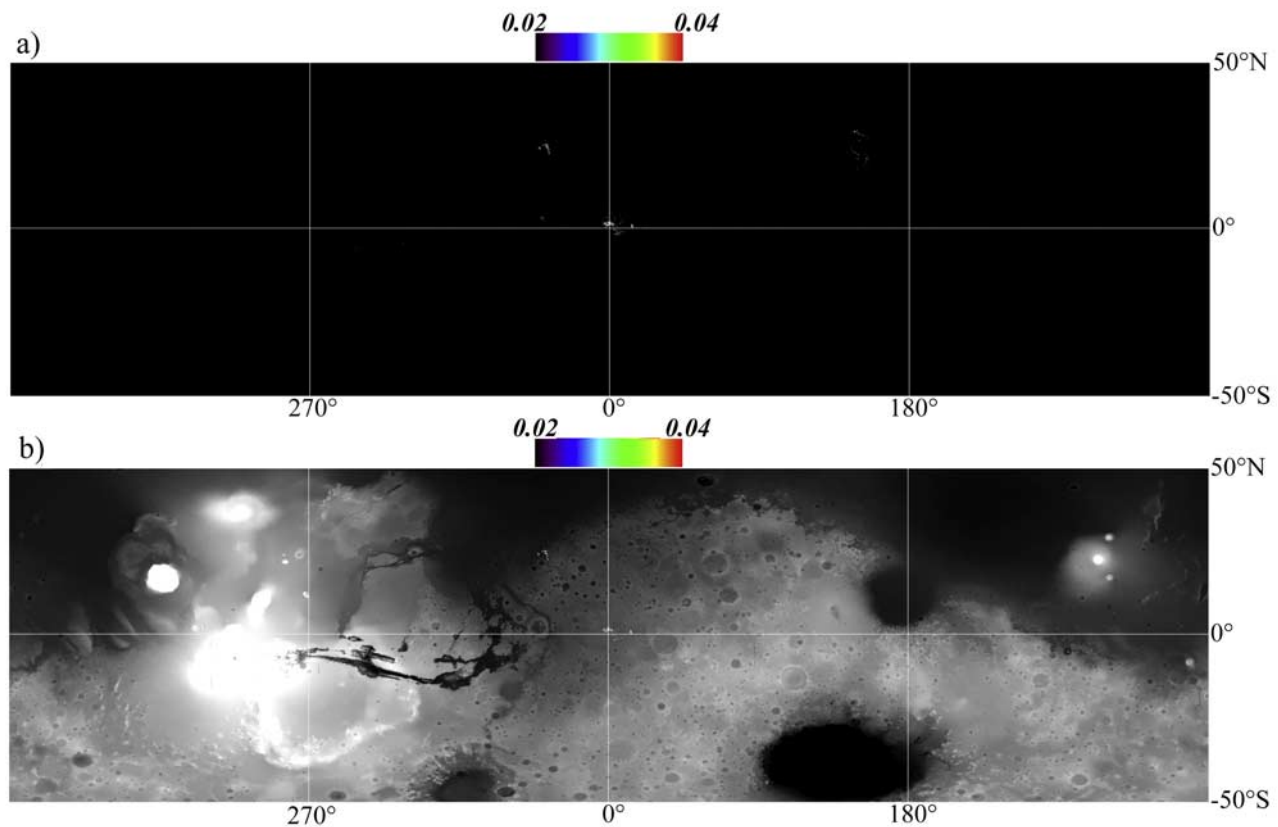
Figure 10. Same as in Figure 6 but for the hydrated minerals identified with the 1.9- \mu\text{m} band criterion.
