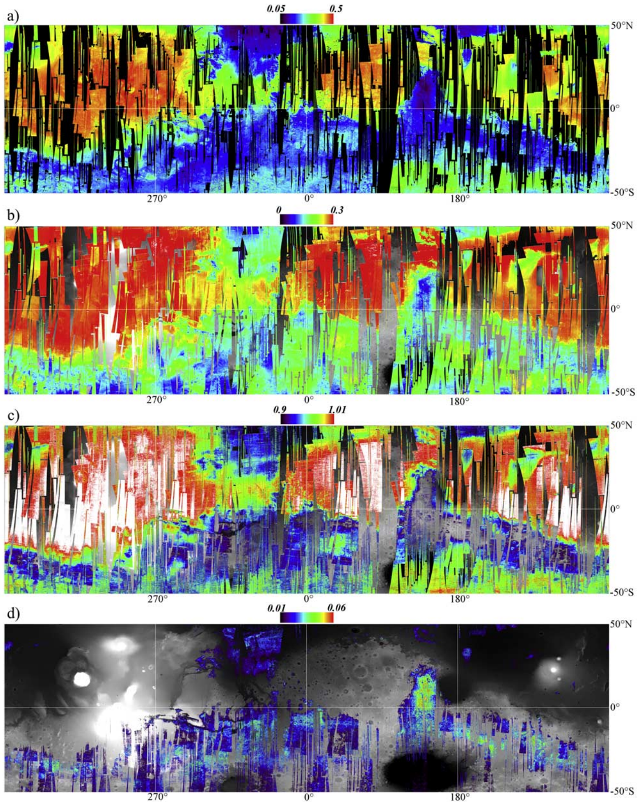
Figure 5. The 32 pixel per degree binned global spectral parameter maps over MOLA map: (a) NIR albedo, (b) Fe 3+ phase, (c) nanophase ferric oxide, and (d) pyroxene. The scales are indicated for each map. Pixels with values below the detection limit are not plotted. Colors that are above the scale are in white.
