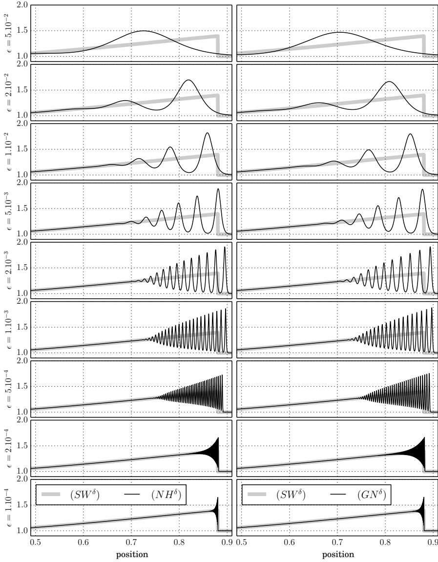
Figure 5: §4.3 Water drop – Rescaled water depth h_l approximated at the rescaled time \sqrt{g\epsilon}t = 0.6 by (NH^\delta) (left column) and (GN^\delta) (right column) for several aspect ratio.
