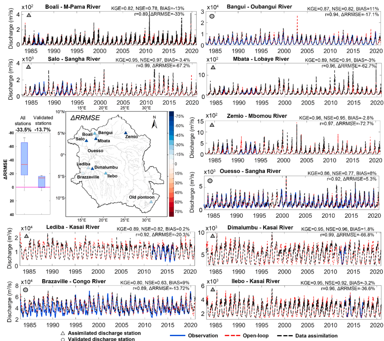
Fig. 9. Time series of observed (blue line), open-loop simulation (dotted red line) and assimilated simulation (dotted black line) discharge for seven assimilated (triangles) and three validated (circles) in-situ stations for the long-term period 1981–2020. The spatial distribution and the boxplot of the \Delta RRMSE performance index for in-situ gauges are shown in the middle-left panel.
