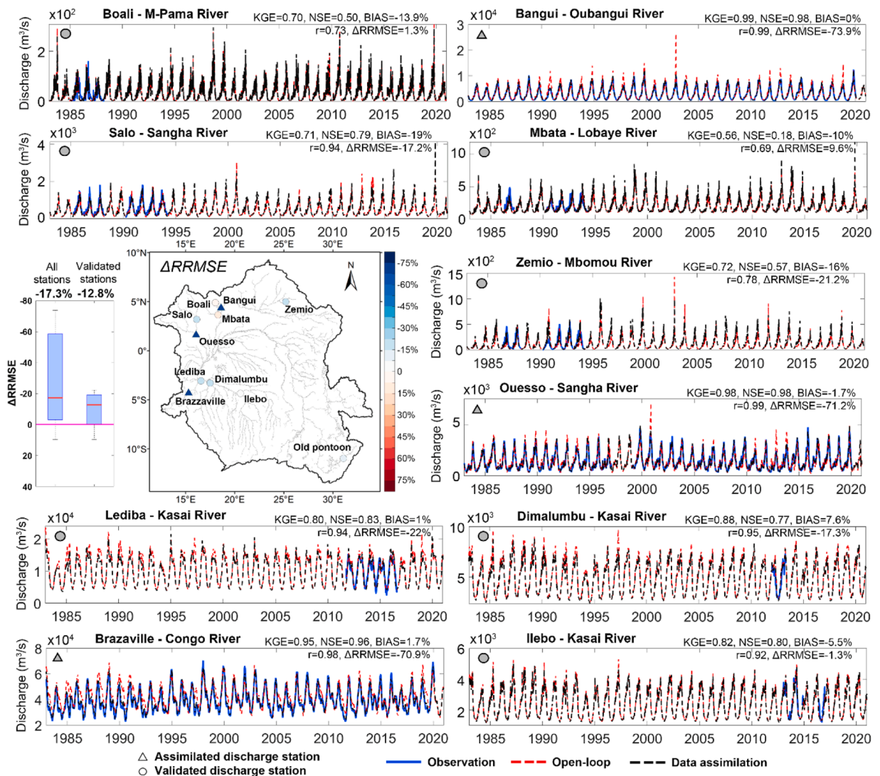
Fig. 8. Time series of observed (blue line), open-loop simulation (dashed red line) and assimilated simulation (dashed black line) discharge for three assimilated (triangles) and seven validated (circles) in-situ stations for the long-term period 1981–2020. The spatial distribution and the boxplot of the \Delta RRMSE performance index for in-situ gauges are shown in the middle-left panel.
