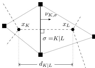
FIGURE 1. Notations of the mesh \mathcal{T} associated with \Omega .
