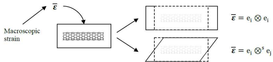
Figure 19. Illustration of the RVE considered in the tensor of stiffness.
