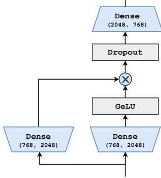
(b) Gated feedforward net.
