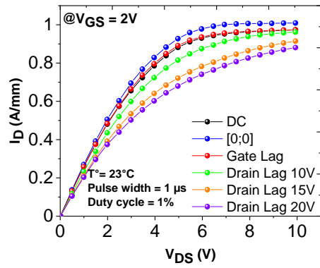
Fig. 2. Open channel I_{\text{D}}\text{-}V_{\text{DS}} output characteristics of 2 \times 50 \mu\text{m} AlN/GaN HEMT for L_{\text{GD}} = 0.5 \mu\text{m} and L_{\text{G}} = 100 \text{ nm} of the structure with high C-doping buffer
