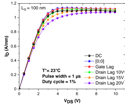
Fig. 4. Open channel I_{\text{D}}\text{-}V_{\text{DS}} output characteristics of 2 \times 50 \mu\text{m} AlN/GaN HEMT for L_{\text{GD}} = 0.5 \mu\text{m} and L_{\text{G}} = 100 \text{ nm} of the structure with medium C-doping buffer + thin AlGaIn BB
