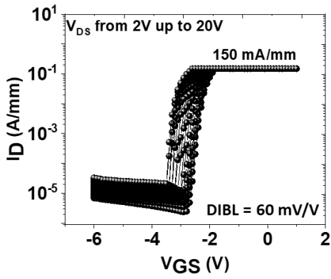
Fig. 1. Transfer characteristics of 2 \times 50 \mu\text{m} AlN/GaN HEMT for L_{\text{GD}} = 0.5 \mu\text{m} and L_{\text{G}} = 100 \text{ nm} of the structure with high C-doping buffer
