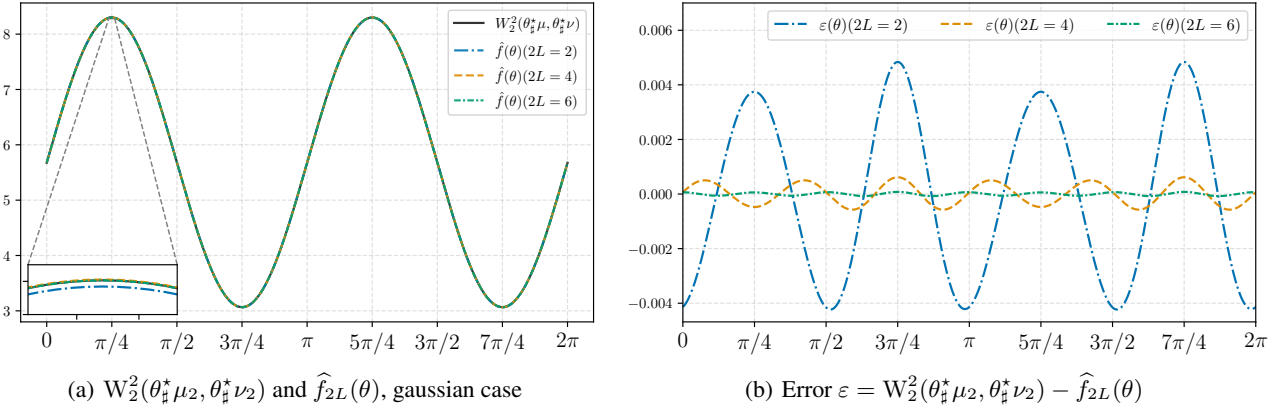
Figure 10. W_2^2(\theta_*^* \mu_2, \theta_*^* \nu_2) , polynomial approximation \hat{f}_{2L}(\theta) and errors \varepsilon = W_2^2(\theta_*^* \mu_2, \theta_*^* \nu_2) - \hat{f}_{2L}(\theta) for two Gaussian measures.
