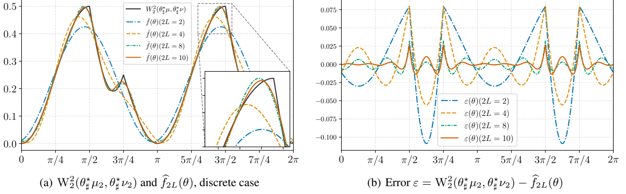
Figure 9. W_2^2(\theta_*^* \mu_2, \theta_*^* \nu_2) , polynomial approximation \hat{f}_{2L}(\theta) and errors \varepsilon = W_2^2(\theta_*^* \mu_2, \theta_*^* \nu_2) - \hat{f}_{2L}(\theta) for two discrete measures.
