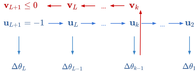
Fig. 1. illustration of the chain rule algorithm.
