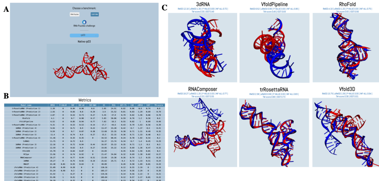
Figure 5. Screenshot of the State-of-the-RNArt dashboard. A: The user can choose the RNA (or challenge) with its native structure to process with the different RNA 3D structure prediction tools. The RNAs are from RNA-Puzzles challenges (79) and from some of the CASP-RNA challenges (83). B: Prediction results were obtained by the nine benchmarked tools and evaluated with different metrics. The metrics are computed with RNAAdvisor (80). C: 3D visualisations of the different predictions of the benchmarked models. The native structure is coloured in red, while the predictions are in blue. The predictions are superimposed with the native structure for visualisation using the US-align (93) tool. The associated metrics are also shown on top of the structures.
