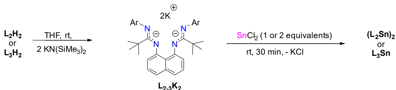
Scheme 3. Synthetic routes to obtain L_{2,3}Sn from deprotonated bis(amidinate) ligands.
