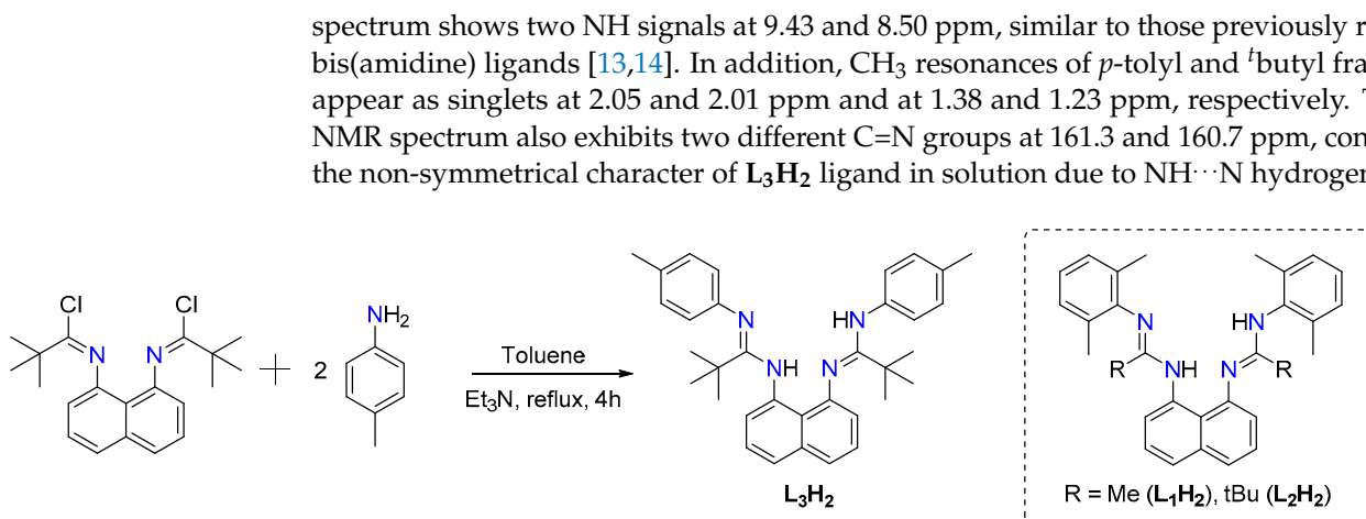
Scheme 1. Synthesis of ligand L 3 H 2 .
