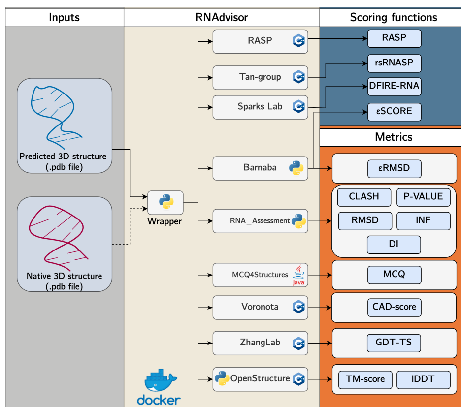
Figure 1. Schema of RNAAdvisor tool: a wrapper code that gathers open-access libraries for assessment of RNA 3D structures in one interface. It is wrapped in a Docker image to emancipate laborious installation processes. A user can input an RNA 3D structure with the reference structure, and it will compute each metric and scoring function using the different integrated software.
