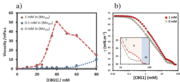
Figure 7. a) Viscosity of \text{Mo}_{154} solutions (for 0, 0.5 mM and 1 mM) with different compositions of C8G1 (0–80 mM). Experiments were performed at 25 °C, and the viscosity of the solutions was measured after incubation for 15 min; b) Surface tension variation at the interface of C8G1 aqueous solution at 298 K showing the influence of 1 mM \{\text{Mo}_{154}\} ring shaped anion upon the classical behavior of the C8G1 surfactant. The shape of \{\text{Mo}_{154}\} -free C8G1 solution giving a cmc value at 23 mM (blue trace) while the presence of \{\text{Mo}_{154}\} 1 mM is highlighted by three domains noted I, II and III (red trace and insert) delimited by two kinks at 18 mM and 57 mM, respectively.
