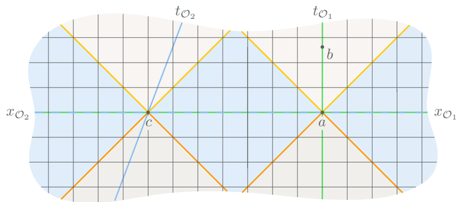
Figure 10: The RPM argument with observer-dependent \varepsilon .
