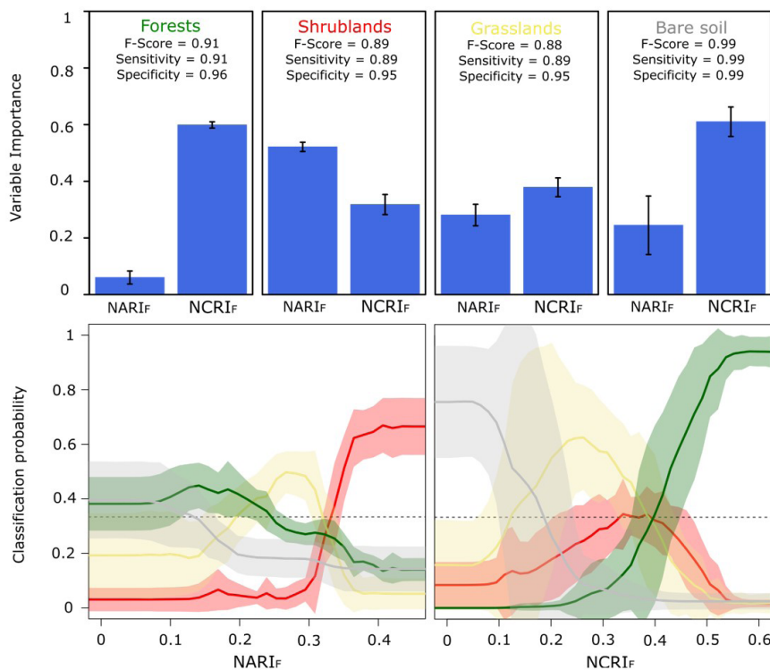
Figure 3. (A) Variables importance in the Random Forest classification for each class with respective F-score, sensitivity and specificity specified. (B) Partial Dependence Plot for NARIF and NCRIF with shown ranges corresponding to variability within the 100 random iterations.
