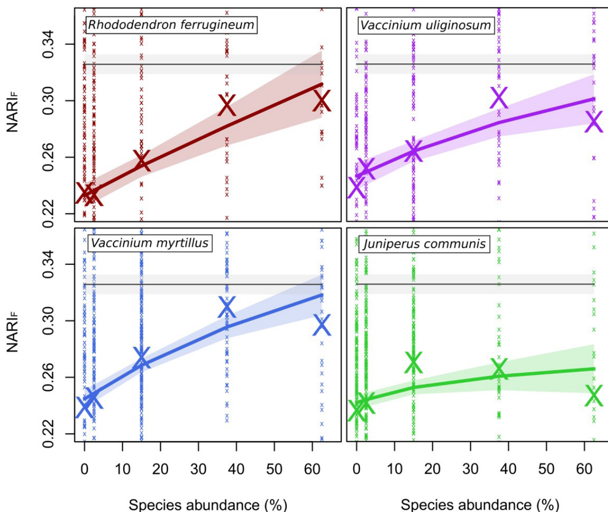
Figure 4. Relation between NARIF and species abundance for Rhododendron ferrugineum , Vaccinium uliginosum , Vaccinium myrtillus and Juniperus communis . Curves correspond to loess fit with span = 2. Confidence interval corresponds to 0.95. Crosses represent mean values for each abundance class. Horizontal gray bars show the NARIF threshold used by the random forest classification to classify a pixel as "shrublands".
