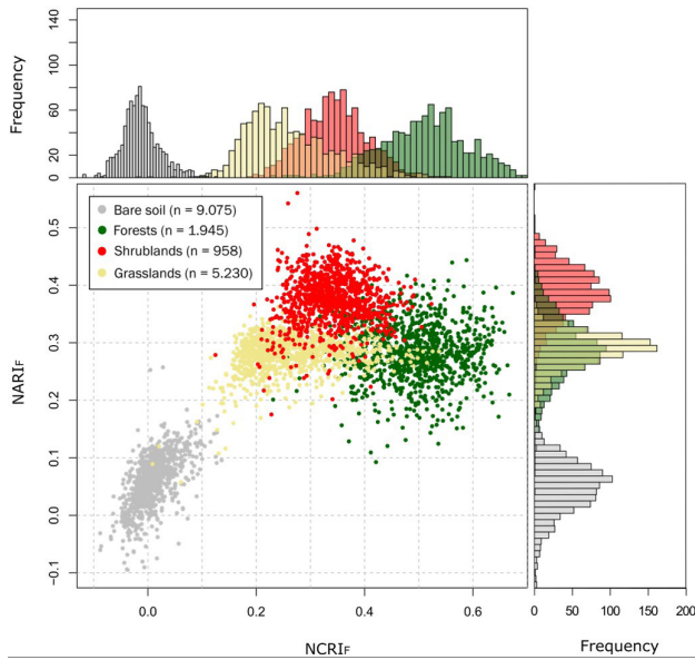
Figure 2. Distribution of training samples for the four classes within the NARIF/NCRIF two-dimensional space.
