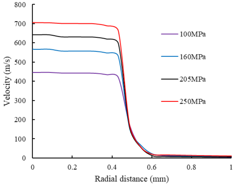
Fig.4 Velocity distribution along radial direction
