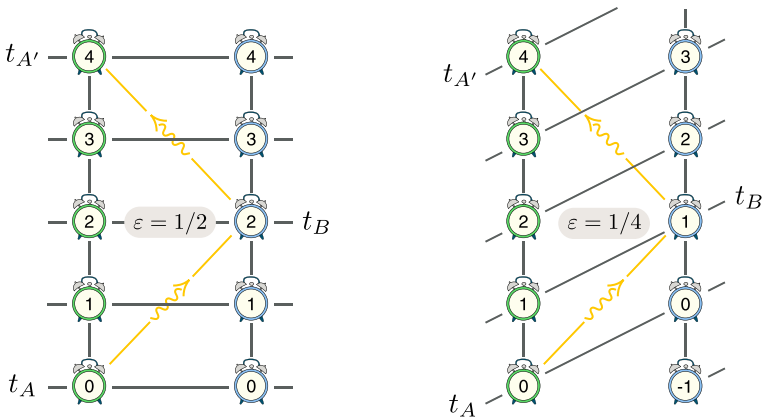
Fig. 2 Standard \varepsilon = \frac{1}{2} versus non-standard \varepsilon = \frac{1}{4} synchrony. Figure adapted from Norton [23]
