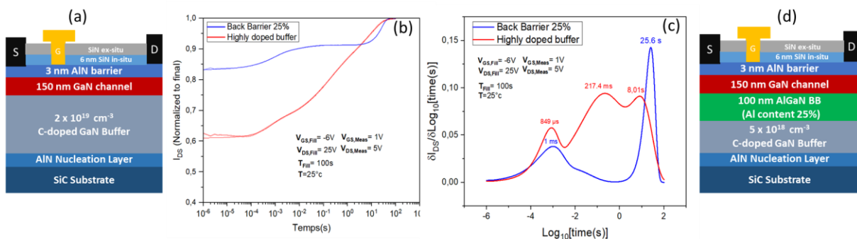
Fig. 1. DCT monitoring subsequent to 100 s filling pulse and corresponding time constants spectrum for AlN/GaN HEMTs with high C-doped GaN buffer and AlGa N back-barrier with low C-doped buffer [1] K. Harrouche et al. , Appl. Phys. Express 2022, 15, 116504.
