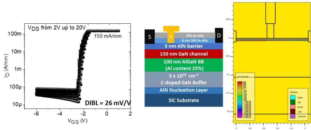
Fig. 3. Transfer characteristics from V_{DS} = 2V up to 20V (left) and TCAD spatial current distribution plot in off-state (right) for the low C-doped buffer and AlGaIn BB structure
