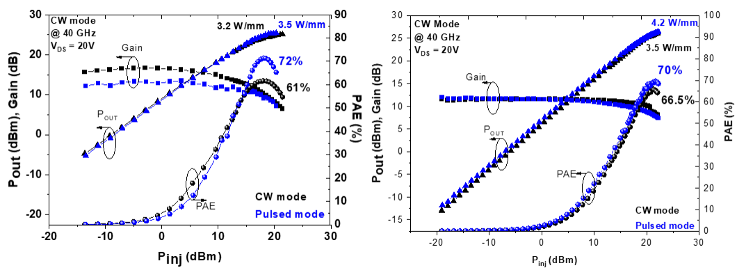
Fig. 4. CW and pulsed large signal performances at 40 GHz for the highly C-doped buffer structure (left) and low C-doped buffer and AlGaIn BB structure (right)
