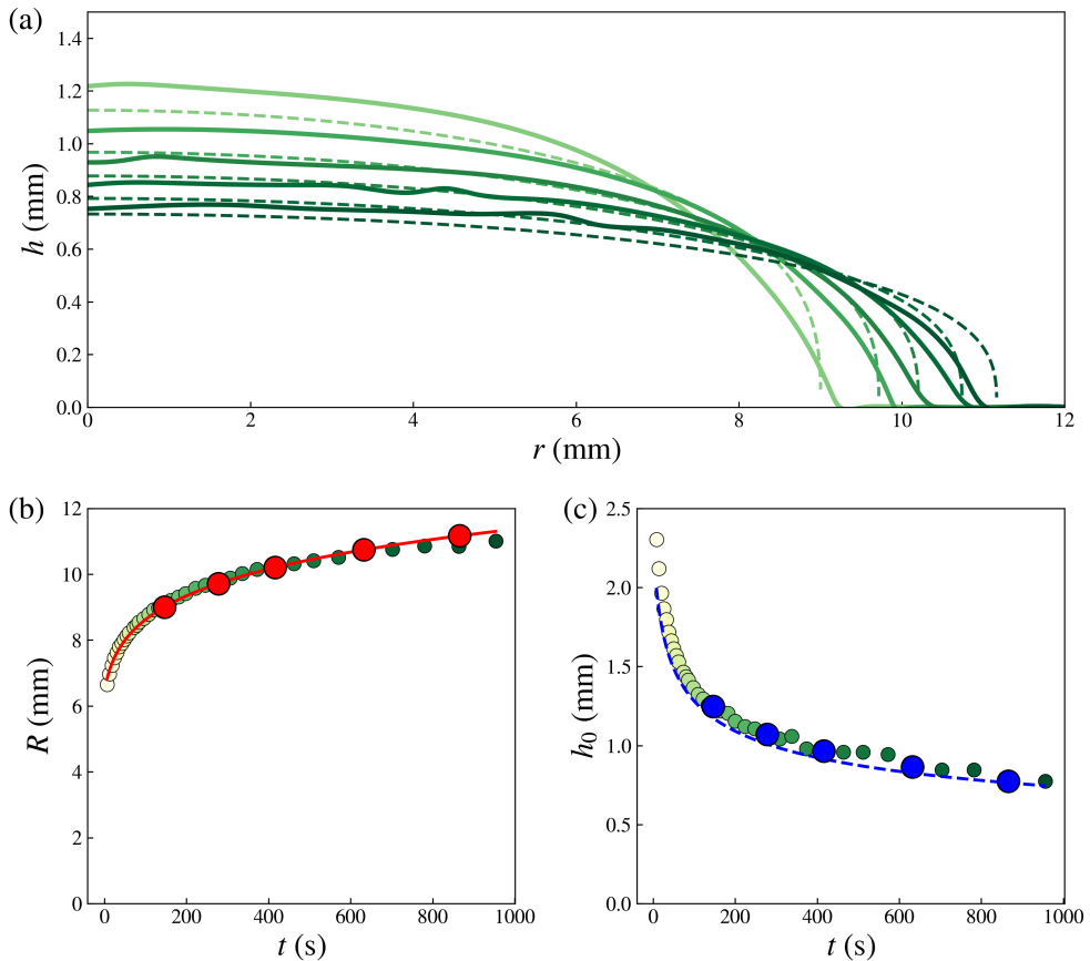
Figure 7: Spreading of a drop of suspension made of a 140- \mu\text{m} particles with V_0 = 215 \mu\text{L} and \phi = 40\% . (a) Experimental profiles from side views (solid lines) and theoretical shapes. Dashed lines: prediction from (3.3) given by Lopez et al. (1976). (b) Dots: experimental radius R as a function of time, red line: power-law growth R = A(t + t_0)^{1/8} , with the fitted parameters A = 4.79 \cdot 10^{-3} \text{ m s}^{-1/8} , t_0 = 10.8 \text{ s} . (c) Central thickness h_0 as a function of time. Dots: measurements from side views, dashed line: prediction of (3.3) using R(t) fitted in subplot (b). The colour gradation indicates the time progression and the large dots in (b) and (c) correspond to the moments of the profiles plotted in (a).
