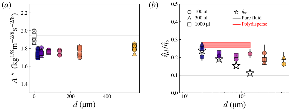
Figure 3: (a) Normalised factor A^* = A(\eta_f/V_0^3)^{1/8} versus particle diameter d (from 20 \mu\text{m} to 550 \mu\text{m} ) for drop volumes of 100 \mu\text{L} , 300 \mu\text{L} and 1000 \mu\text{L} . The white open symbols correspond to experiments with pure fluid. (b) Ratio of the relative effective viscosity obtained from the power law, \hat{\eta}_d , to the relative bulk viscosity, \hat{\eta}_s , versus particle diameter d . The red horizontal line corresponds to this ratio for a polydisperse suspension made of particles of 20 \mu\text{m} , 40 \mu\text{m} , 80 \mu\text{m} and 140 \mu\text{m} , each size representing 10 % of the suspension volume. The star symbols correspond to the relative effective wetting viscosity of the same suspensions obtained from the Cox-Voinov law, \hat{\eta}_w (Zhao et al. 2020).
