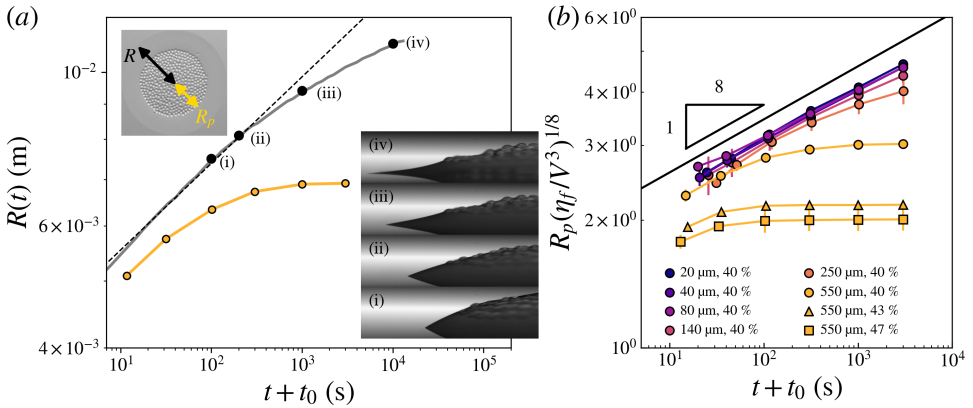
Figure 6: (a) Drop of suspension consisting of 550- \mu\text{m} particles with V_0 = 100 \mu\text{L} . Main graph: fluid radius R (black) and particle radius R_p (yellow) as a function of time. The dashed line corresponds to the power law. Thumbnails (i) to (iv): side-view pictures corresponding to the black dots in the main graph. Top inset: top view picture with fluid ( R ) and particle ( R_p ) radii. (b) Particle radius R_p as a function of time for different suspensions (see legend) with a drop volume V_0 \approx 100 \mu\text{L} . Error bars are computed from standard deviations over different experiments.
