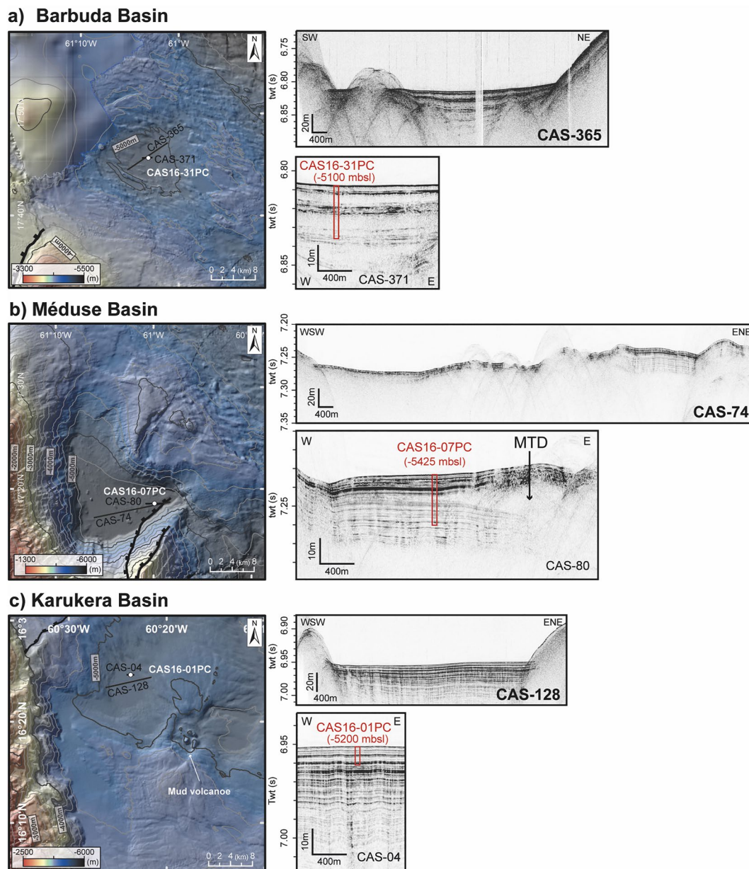
Figure 3. Maps (Located on Figure 1b) and Sub Bottom Profiles (SBP) of the Barbuda Basin (a), Méduse Basin (b) and Karukera Basin (c). The SBP CAS-371, CAS-80 and CAS-04 were acquired with the research vessel drifting with propellers turned off to lower the noise. The red rectangles on the SBP correspond to the location and penetration of the core into the basins.
