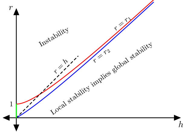
Figure 5: This figure shows the stability regions in the (h, r) -plane. The red curve is r = r_1 , which represents the solution of \bar{y}_h = 1 + h , while the blue curve is r = r_2 , which represents the solution of H^* = H^*f(H^*) + h . We have local stability in the region below r = r_1 , but the embedding technique fails to address global stability when r_2 < r < h . However, we conjecture that we also obtain global stability when r_2 < r < r_1 . Observe that global stability in the green part of the r -axis, i.e., h = 0 and 0 < r < 1 has been addressed in [15].
