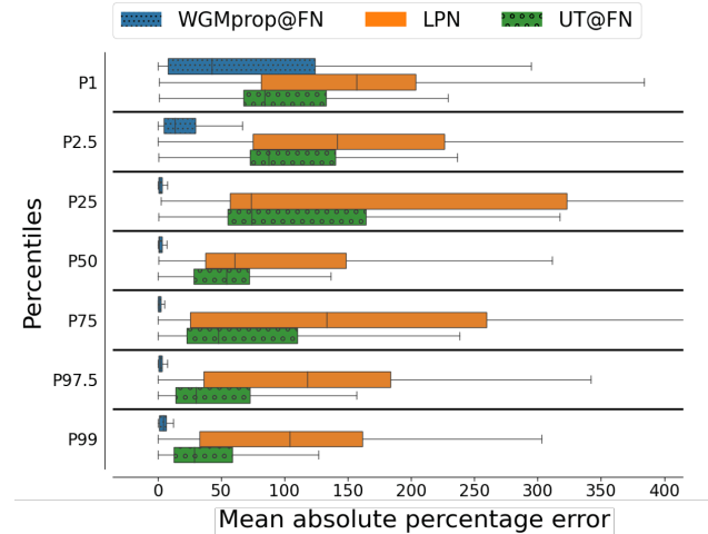
Figure 4. MAPE boxplots for percentiles 1, 2.5, 25, 50, 75, 97.5 and 99. Input images were degraded by a large contrast kernel ( I_3 ).
