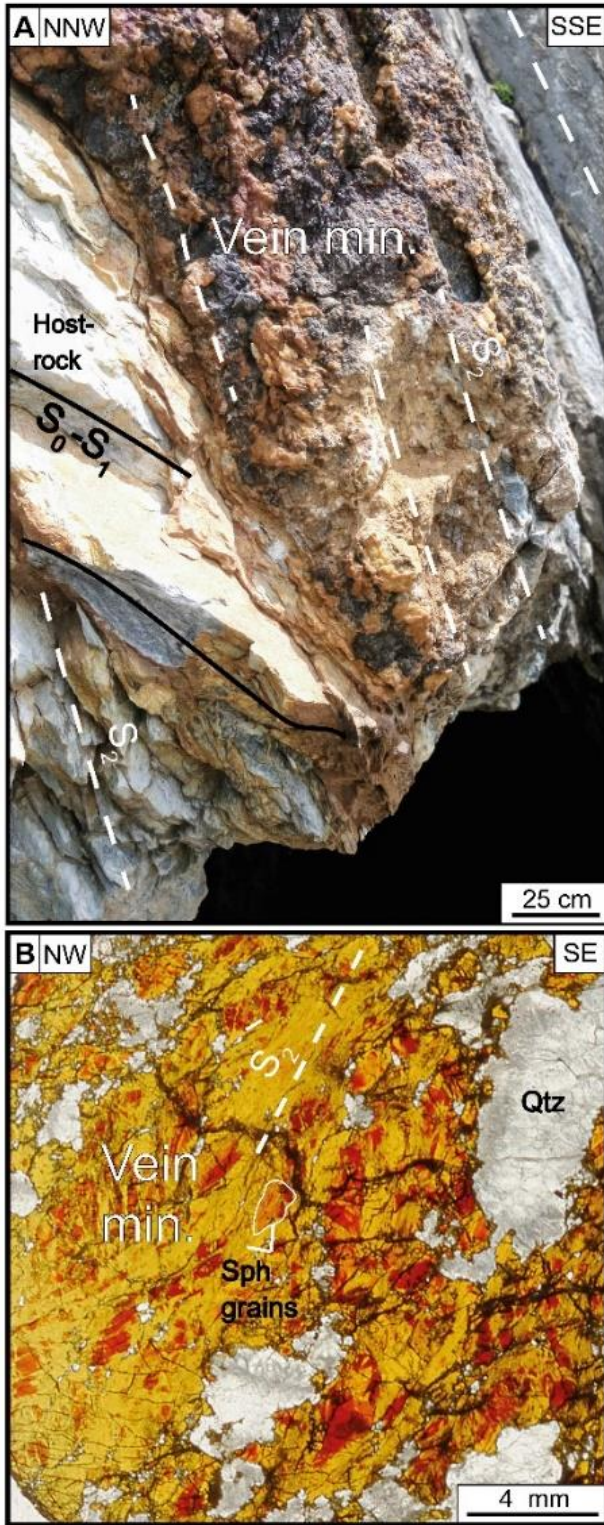
Figure 2: A: Pb-Zn Type 2b Vein in Arre deposit. B: Typical Pb-Zn Type 2b ore mineralization with color zonation in sphalerite and presence of superimposed S 2 cleavage (modified from Cugerone et al., 2018b; S 0 -S 1 : S 0 -S 1 foliation; S 2 : S 2 foliation; Qtz: quartz; Sph: sphalerite).
