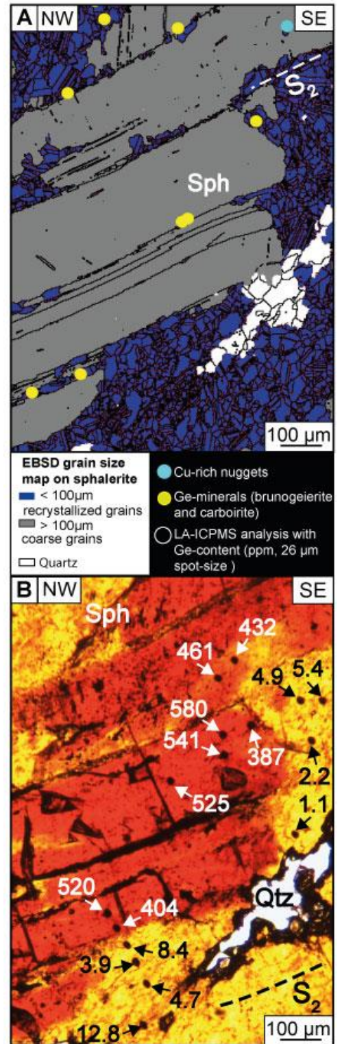
Figure 3: A: EBSD grain size map in sphalerite (Arre sample) with location of Ge and Cu rich phases. These minerals are preferentially located in recrystallized sphalerite domains. B: Corresponding area in transmitted light with LA-ICP-MS spot analyses associated to Ge-contents (in ppm). Note that the contrasts in color observed in Sph correspond to variations in Ge content. (S 2 : S 2 foliation; Qtz: quartz; Sph: sphalerite).
