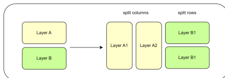
Figure 3: Tensor parallelism applied to 2 layers A et B
