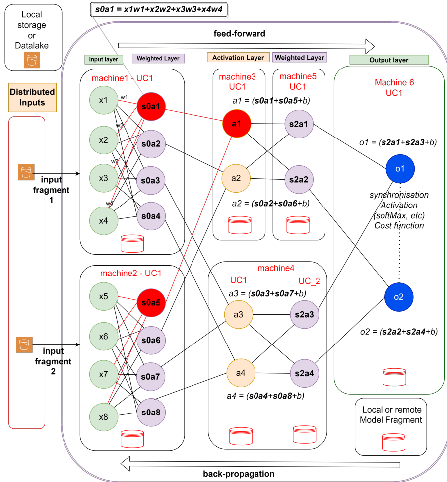
Figure 5: Activation layer in machine3-UC1 waiting for Weighted matrix from 2 UCs machine1-UC1 , machine2-UC1
