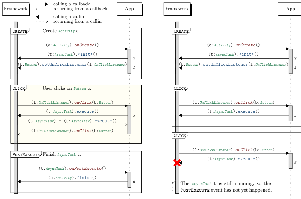
(4.a) A trace that does not witness a protocol violation since the callin (t:AsyncTask).execute() sequences witnesses the no-execute-call-on-already-executing-AsyncTask protocol violation.
