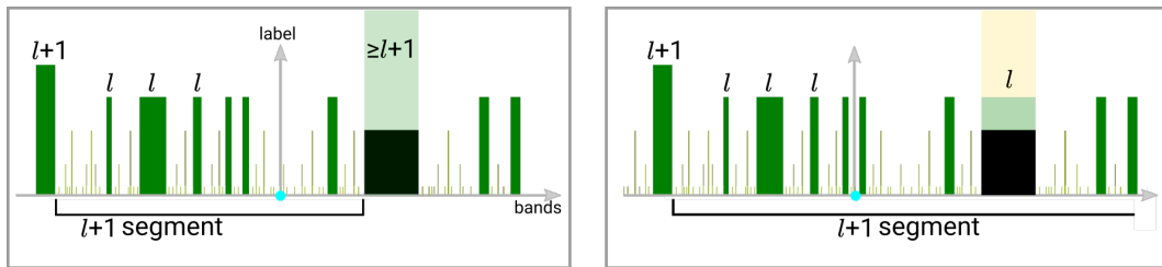
Figure 10: Left: The origin does not lie on the inside of its l + 1 segment since it is too close to the right band of label \geq l + 1 (under the sequence \tilde{N}^{(x)} ). The label of that band has been raised in the construction of Lemma 4.13 (indicated in light green). However, Lemma 4.11 tells us that for infinitely many l , the label under N^{(x)} is lower than that (black portion). Right: We can lower the value of the band to l without changing the band structure but still being larger than N^{(x)} . Then, the l + 1 segment containing 0 becomes larger and 0 is now on the inside of its l + 1 segment.
