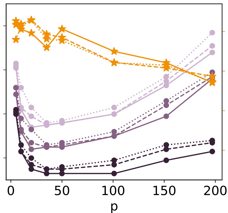
Bubbles with 10 days temporal clustering
