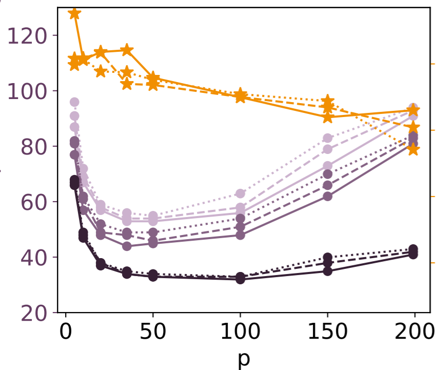
Bubbles with 5 days temporal clustering
