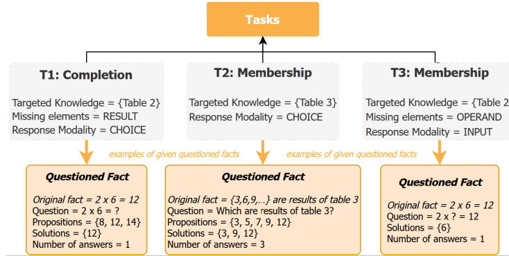
Fig. 4: Examples of questioned facts in generic form.
