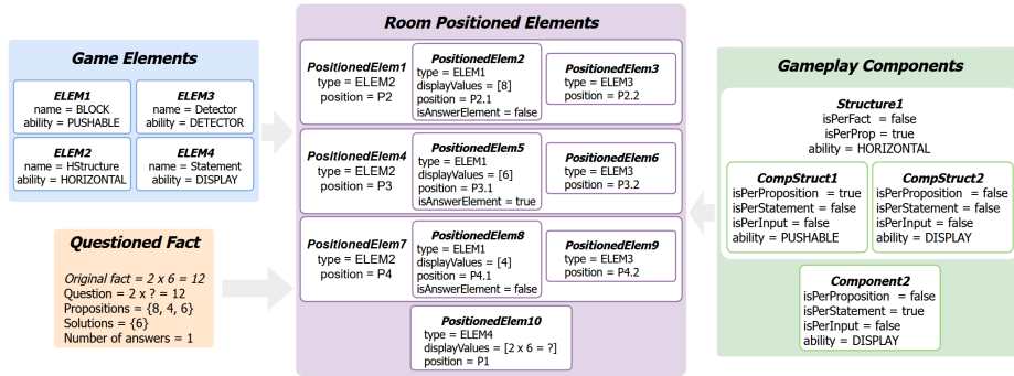
Fig. 7: Example of generated positioned elements.
