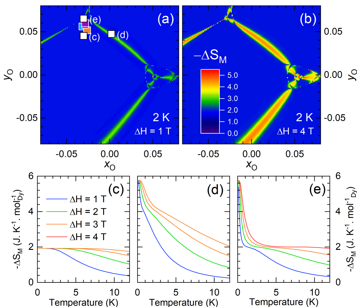
Figure 9 (color online) : (a) and (b) illustrate the variation of -\Delta S_M(2\text{K})_{\Delta H=1\text{T}} and -\Delta S_M(2\text{K})_{\Delta H=4\text{T}} with (x_O, y_O) (in \text{J} \cdot \text{K}^{-1} \cdot \text{mol}^{-1}_{\text{Dy}} ). The color scale is the same in both (a) and (b). The colored square symbols correspond to the (x_O, y_O) coordinates of the garnets synthesized for this work. (c) to (e) show the theoretical magnetic entropy variation -\Delta S_M , calculated from the magnetic
