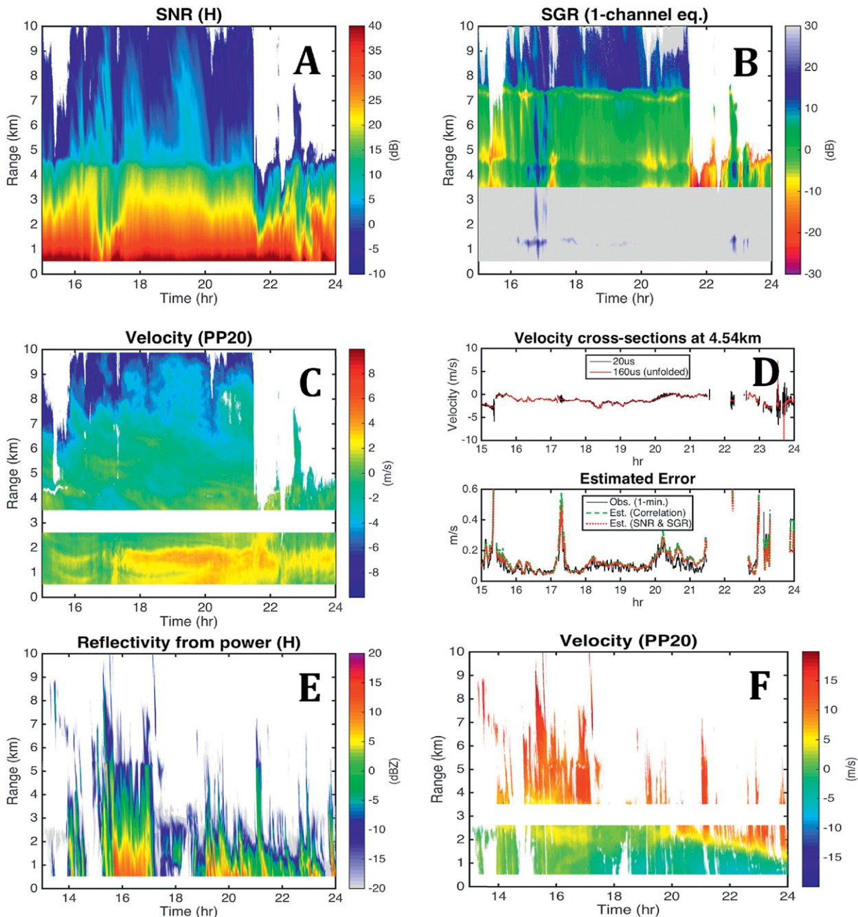
FIG. 8. Observations at Chilbolton at 45^\circ elevation showing the increased random error in the velocity estimates due to ghosts on 27 Jun 2017: (a) the SNR in the H channel; (b) the SGR in the H channel due to the depolarization of the V channel shifted by 3 km in range; (c) PP20, which is the velocity derived from the H–V [20 \mu\text{s} (3 \text{ km})^{-1}] pulse pairs with a folding velocity of 40 \text{ m s}^{-1} ; and (d) top trace showing the “true” velocity (red line) derived from a pulse separation of 160 \mu\text{s} at a height of 4.54 km and the PP20 velocity from the H–V pulses (black). Note the increased noise in the black trace when SGR and SNR are low. The bottom trace in (d) shows the observed rms error obtained by comparing the true PPI60 velocity with the PP20 H–V velocity (black), and the close agreement with the theoretical errors from the SNR and SGR (red), and from the H–V correlation (green). (e),(f) The high wind shear case accompanied by large vertical reflectivity gradients observed on 28 Aug 2017. For details see the text.
