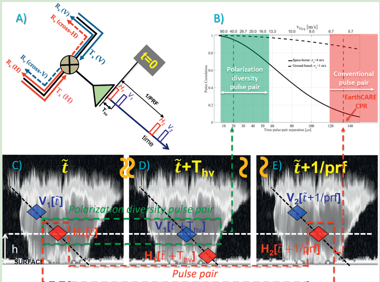
FIG. SB1. A high Doppler folding velocity is needed to measure atmospheric winds. At 94 GHz, this is achieved by transmitting two closely spaced pulses, one with horizontal polarization and the other vertical.
