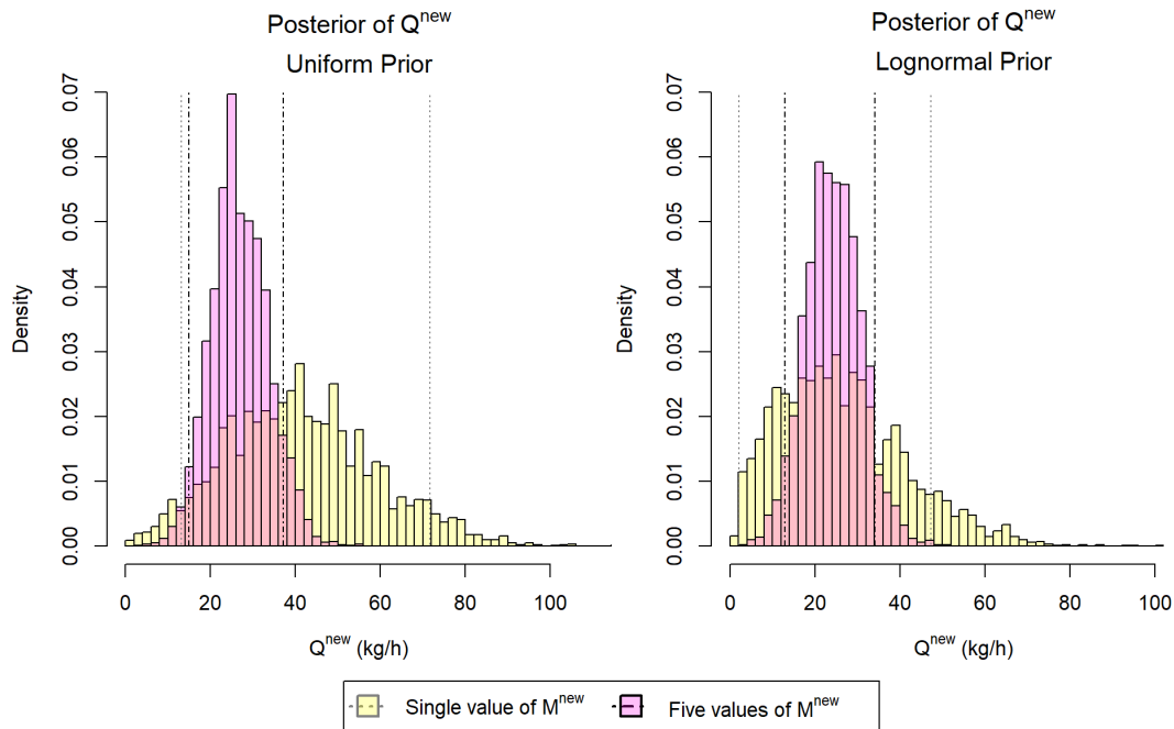
Figure 11: Posterior distributions for the true value of the emission rate given the observed measurement(s), prior distribution, and controlled release data.
