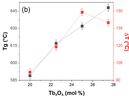
Fig. 4. a. DSCs curves and b. Tg and ΔT obtained for samples with different contents of Tb 2 O 3 in the ternary system.
