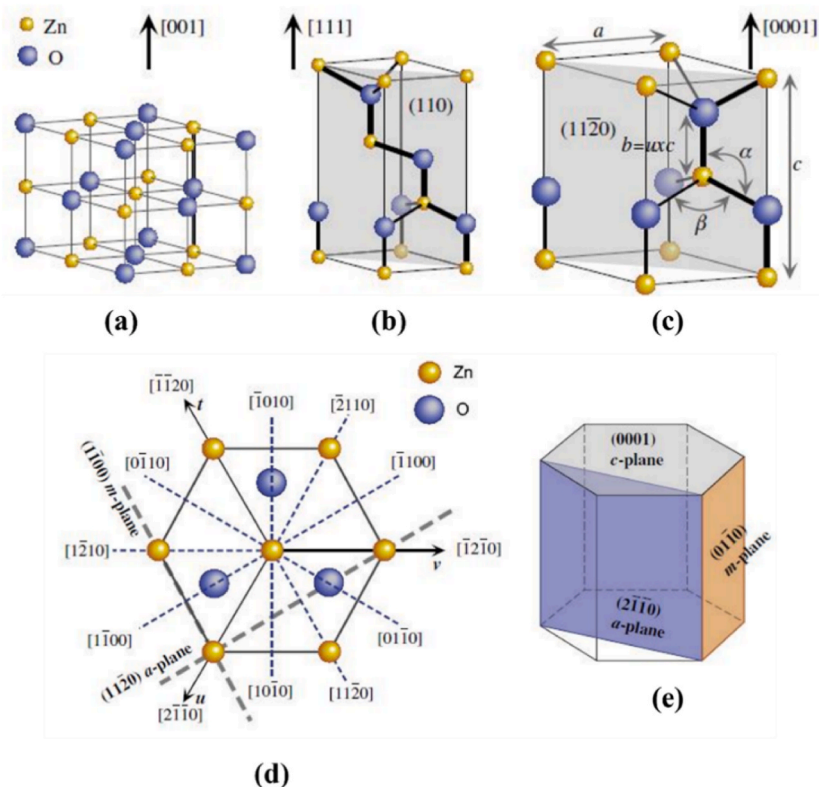
Fig. 1. Schematic of ZnO crystal structures: (a) CRS, (b) cubic ZB, and (c) HW. (d) Various crystal planes of hexagonal würtzite structure and (e) 3D view of hexagonal würtzite unit cell. Adapted from Ref. [37]. Copyright 2023 Elsevier.
