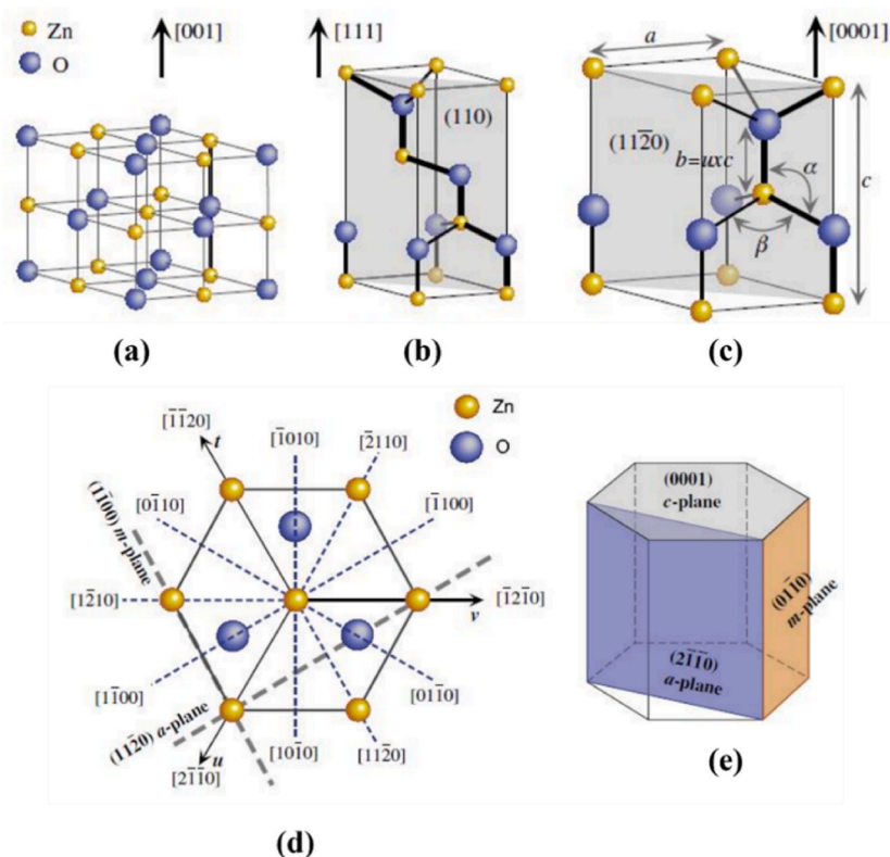
Fig. 1. Schematic of ZnO crystal structures: (a) CRS, (b) cubic ZB, and (c) HW. (d) Various crystal planes of hexagonal wurtzite structure and (e) 3D view of hexagonal wurtzite unit cell. Adapted from Ref. [37]. Copyright 2023 Elsevier.
