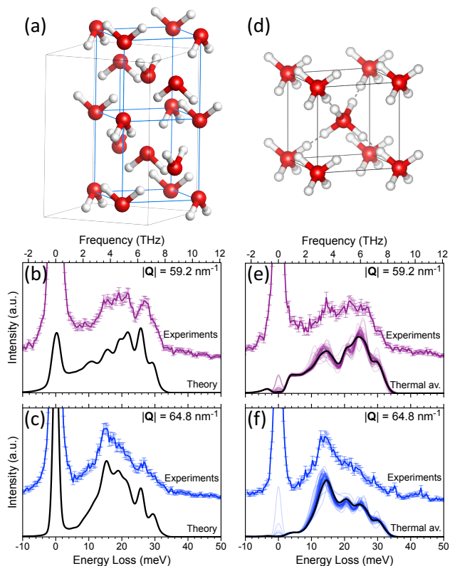
FIG. 1. (Color online) Structure of tetragonal ice VIII in (a) and cubic ice VII in (d) with oxygen drawn in red and hydrogen sites in white. In ice VII, the 4 possible hydrogen sites around an oxygen atom are occupied only 50% averaged over space and time. On the contrary, in ice VIII the H-site is 100% occupied. In (a), the unit cell of ice VIII is drawn in black and the associated unit cell of ice VII in blue. Examples of constant- |\mathbf{Q}| scans (colored lines with error bars) of ice VIII in (b)-(c) and ice VII in (e)-(f) collected at 30 K and ambient pressure. Experiments are compared to first-principle calculations (thick black lines). For ice VII, the average spectrum is superimposed to the 52 supercell contributions (thin colored lines). A Gaussian broadening of full width at half maximum of 1.7 meV was employed to account for the instrumental energy resolution.
