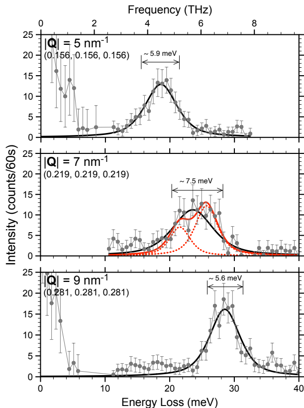
FIG. 4. IXS spectra recorded at 300 K on a single crystal of ice VII at 2.6 GPa along the [111] direction, in the region of the predicted gap. \mathbf{Q} -point coordinates are given in 2\pi/a unit where a is the lattice parameter of the unit cell. Black lines are used to represent the fits performed with a single pseudo-Voigt. In the case of |\mathbf{Q}| = 7 \text{ nm}^{-1} , an additional fit with two pseudo-Voigt functions is shown in red to mimic the presence of a gap.
