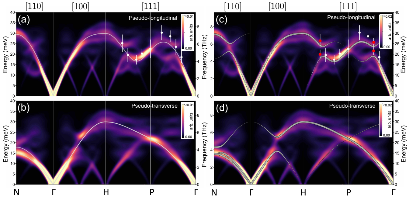
FIG. 3. Phonon dispersion of ice VII. The color-coded intensity map corresponds to ensemble-averaged \langle S_{\hat{n}}^{\text{OO}}(\mathbf{Q}, \omega) \rangle along high symmetry directions of the extended Brillouin zone of the oxygen body-centered cubic sublattice. The unit vector \hat{n} was chosen to be either parallel to \mathbf{Q} to reveal the longitudinal character of phonon modes in (a) and (c) or perpendicular to \mathbf{Q} to reveal the transverse character of the modes in (b) and (d). The dispersion obtained when describing ice VII as a monoatomic bcc crystal using a very simple Born-von Kármán model is superimposed (white lines) in (a) and (b). The phonon dispersion of a refined model describing ice VII as two interpenetrating diamond sublattices unfolded in the extended Brillouin zone of the bcc oxygen sublattice (grey circles) is shown in (c) and (d). Energies and full width at half-maximum extracted from fitting the spectra acquired on a single crystal with a single pseudo-Voigt (white dots) are shown in (a) and using two pseudo-Voigt functions (red dots) for |\mathbf{Q}| = 7 and 26 \text{ nm}^{-1} in (c).
